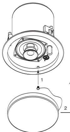
Figure 20: Attach the grille
