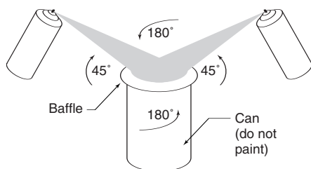
Figure 21: Spray-painting angles
