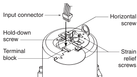
Figure 13: Plug connector into socket
