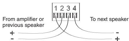
Figure 10: Daisy-chain wiring
