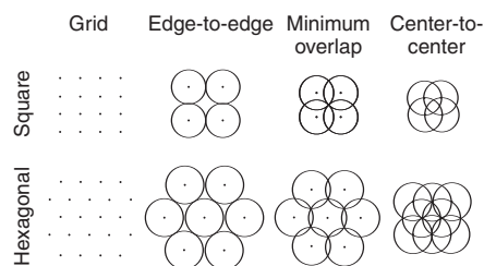
Figure 22: Coverage patterns
